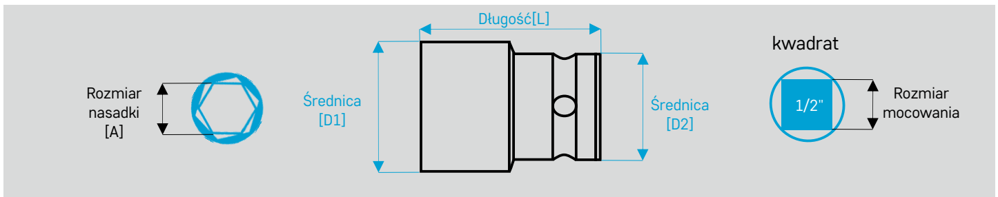
Nasadki udarowe 6-kątne hexagon fast lead
