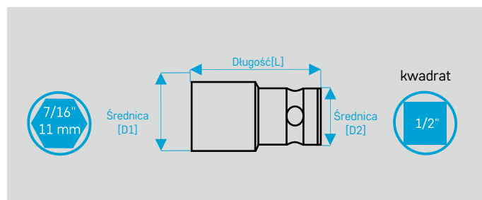
Adaptory 6-kątne hexagon 7/16" - 11 mm
