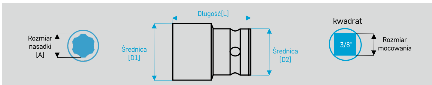
Nasadki udarowe 6-kątne hexagon Surface Drive TORX® PLUS
