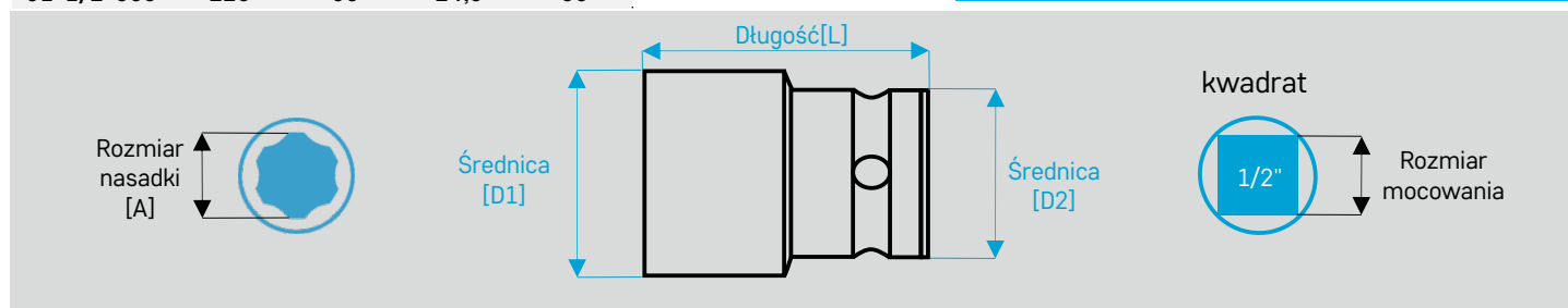
Nasadki udarowe 6-kątne hexagon Surface Drive TORX® PLUS
