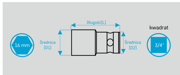
Adaptory 6-kątne hexagon 16 mm
