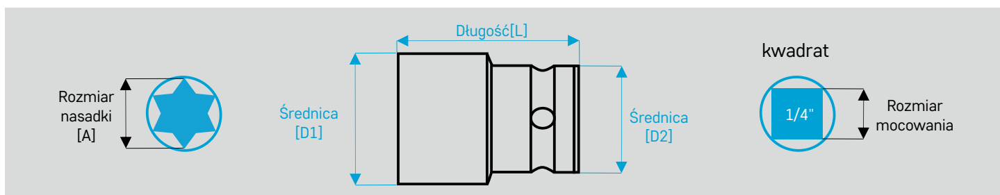
Nasadki udarowe TORX® socket screws
